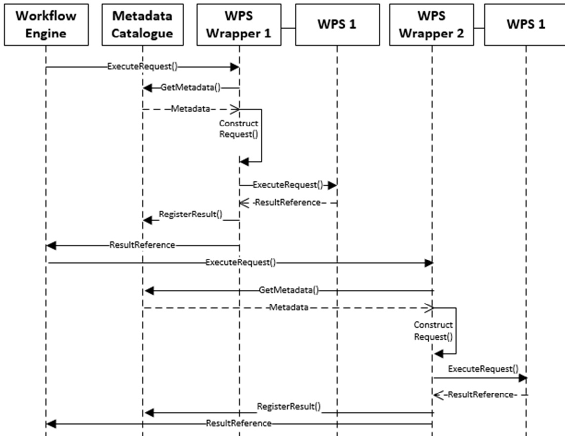
Figure 2: UML sequence diagram of WPS profile workflow
